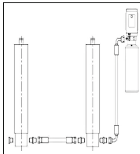
Picture 10 Hydraulic Connections
